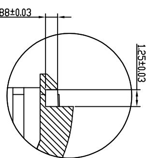
DETAIL D SCALE 5:1
